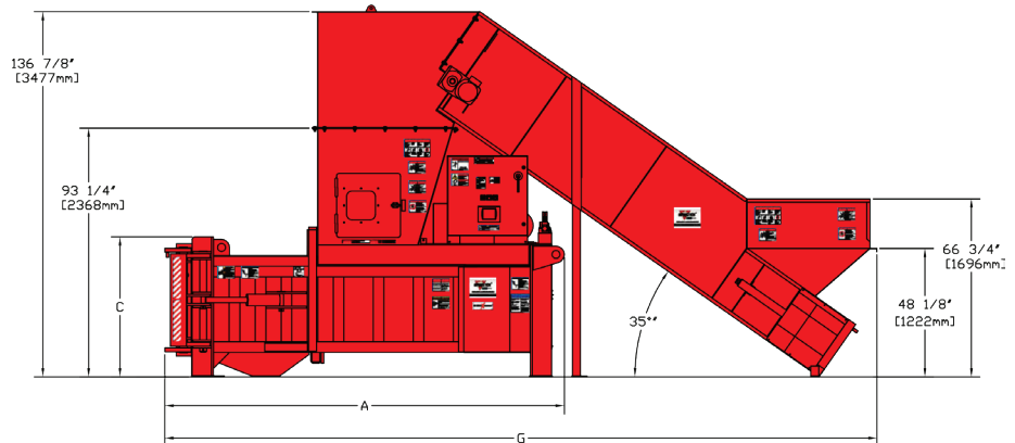
SIDE VIEW
